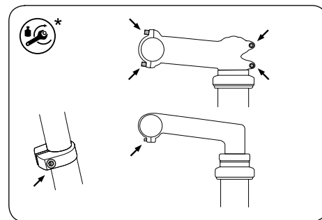
Possible positions for adjusting bolted connections
